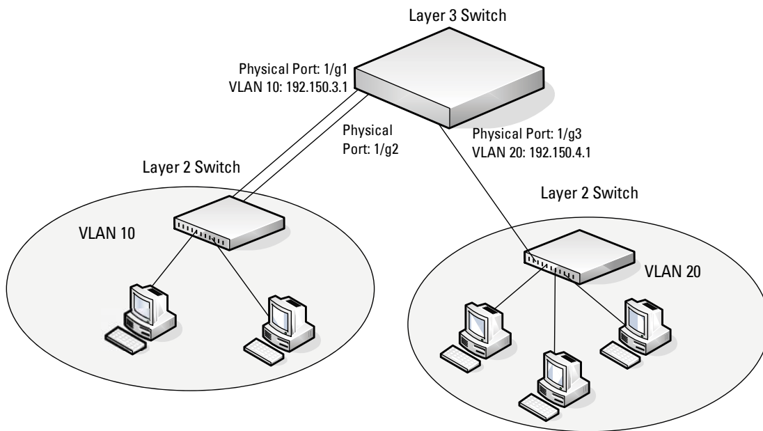
Figure 4-1. VLAN Routing Example Network Diagram
