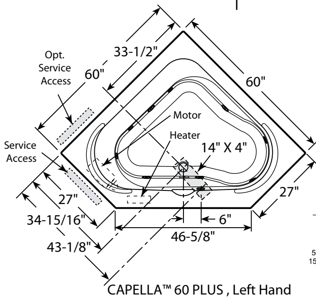
Product Shown: Capella™ Left Hand Motor Plus Whirlpool Bath LH. Model: EN00 * Measurements inside unit represent cutout in floor to allow for drain/overflow. Minimum Service Access dimensions given.
