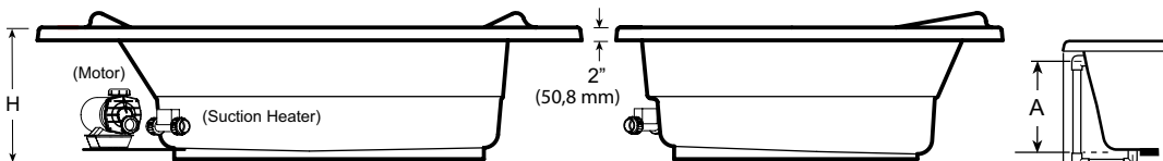
SIDE VIEW
