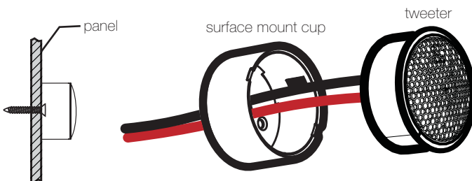
Fig. 4 Surface Mounting
