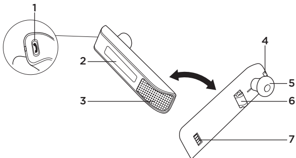
Figure 1: BH870 Wireless Bluetooth Headset diagram
