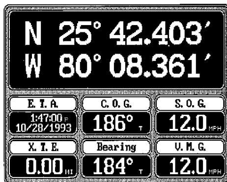
NAVIGATION SCREEN
