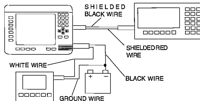
GLOBALMAP 1000 RECEIVING NMEA 0183, VERSION 2.0 DATA FROM NAVIGATION RECEIVER AND SENDING NMEA 0183, VERSION 1.5 DATA TO ANOTHER DEVICE.
