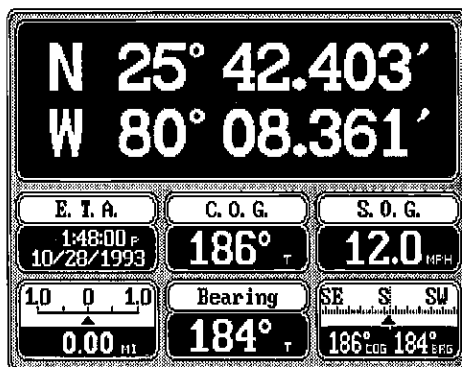
NAVIGATION SCREEN
