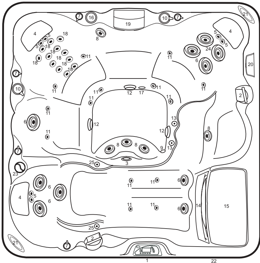
Figure-F, Hot Tub Top View
