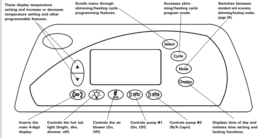
Figure-D, Command Center
