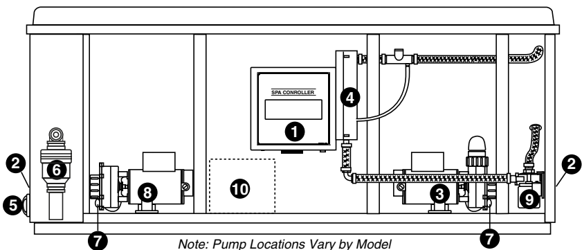
Figure-A, Equipment Area
