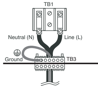
Figure-C, Terminal Block TB1 230V Wire Connection
