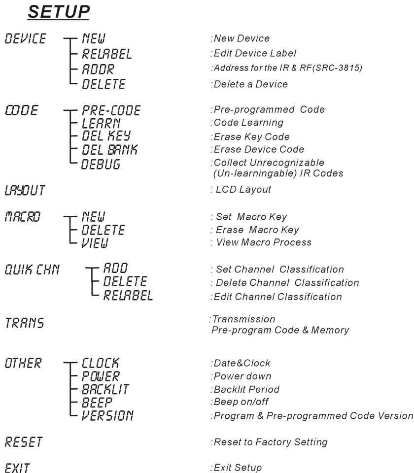
Figure 5: Setup Menu Hierarchy
