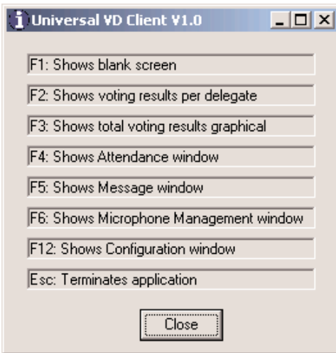
Fig. 5 - Help window.
