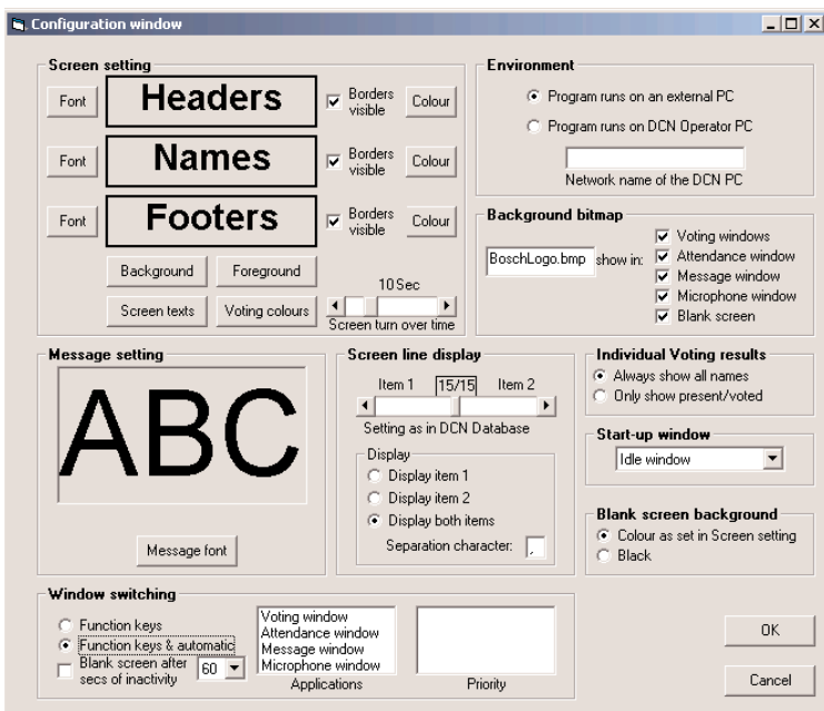
Fig. 2 - Configuration window.
