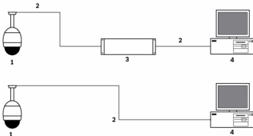
Figure 2.1 AutoDome 700 Series System Configuration
