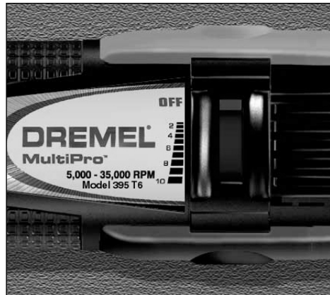
The Settings for Approximate Revolutions Per Minute Rotary Tool Variable Speed Model 395T6.
