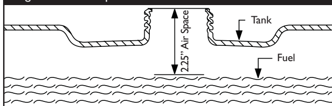
Figure 3 - Fuel Expansion
