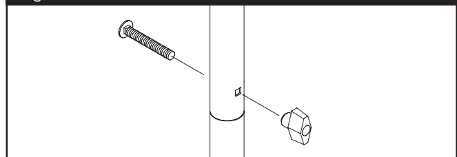
Figure 2 — Secure Handle
