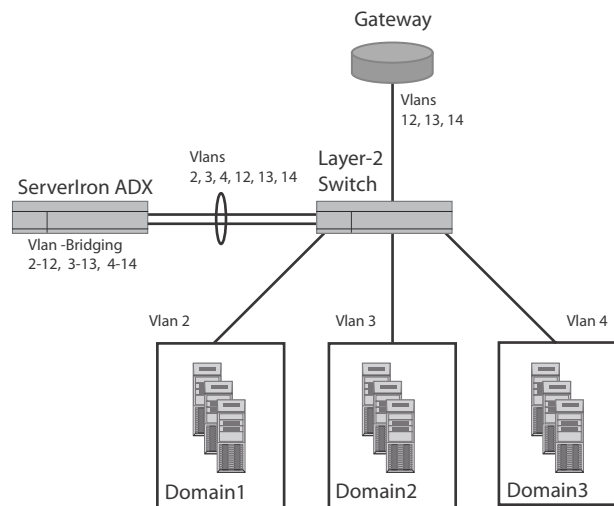
FIGURE 1 VLAN bridging in a one-armed topology
