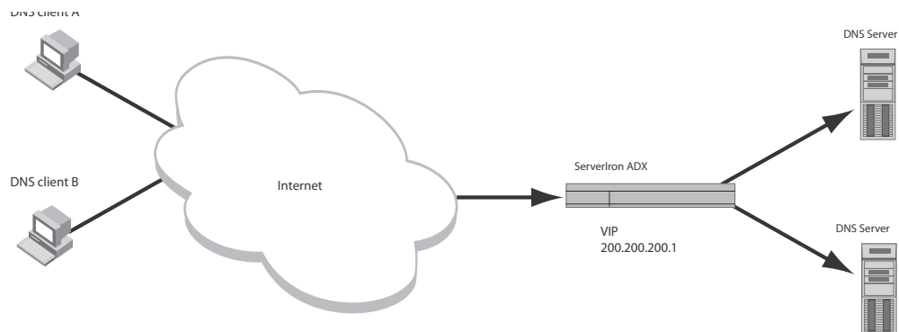
FIGURE 4 DNS attack protection
