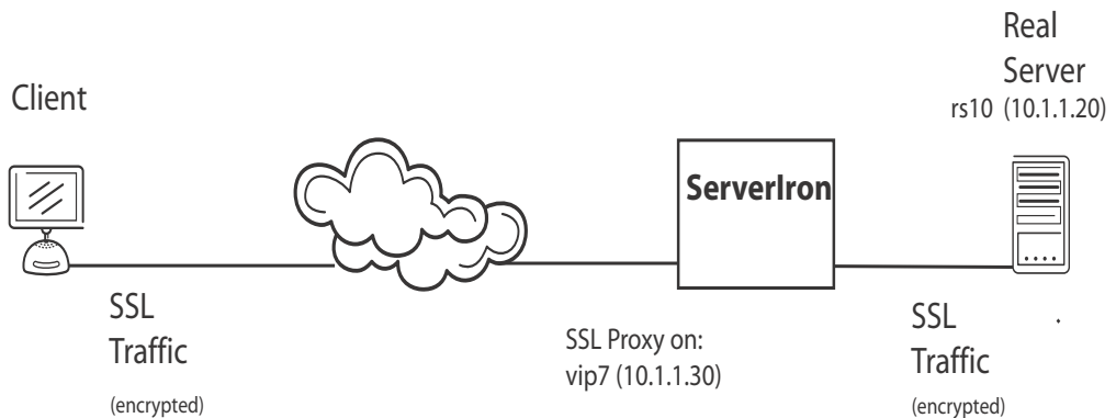
FIGURE 10 ServerIron ADX SSL Proxy
