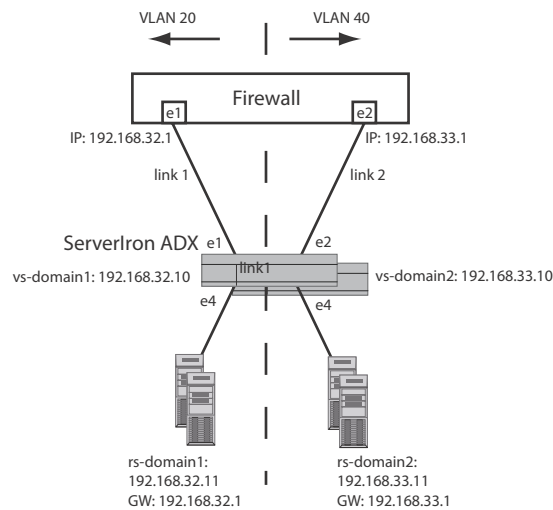
FIGURE 3 Traffic Segmentation
