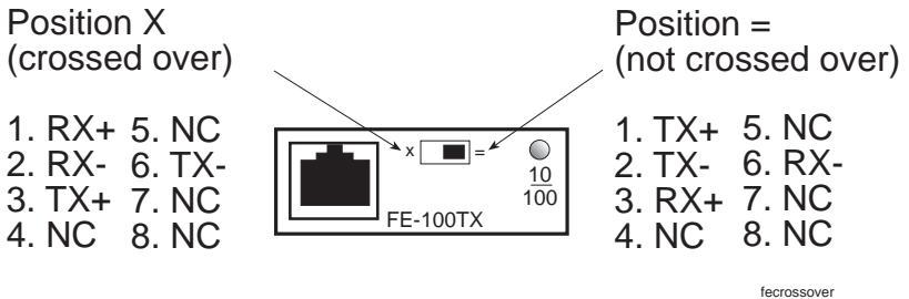
Figure B-1 FE-100TX Pinouts
