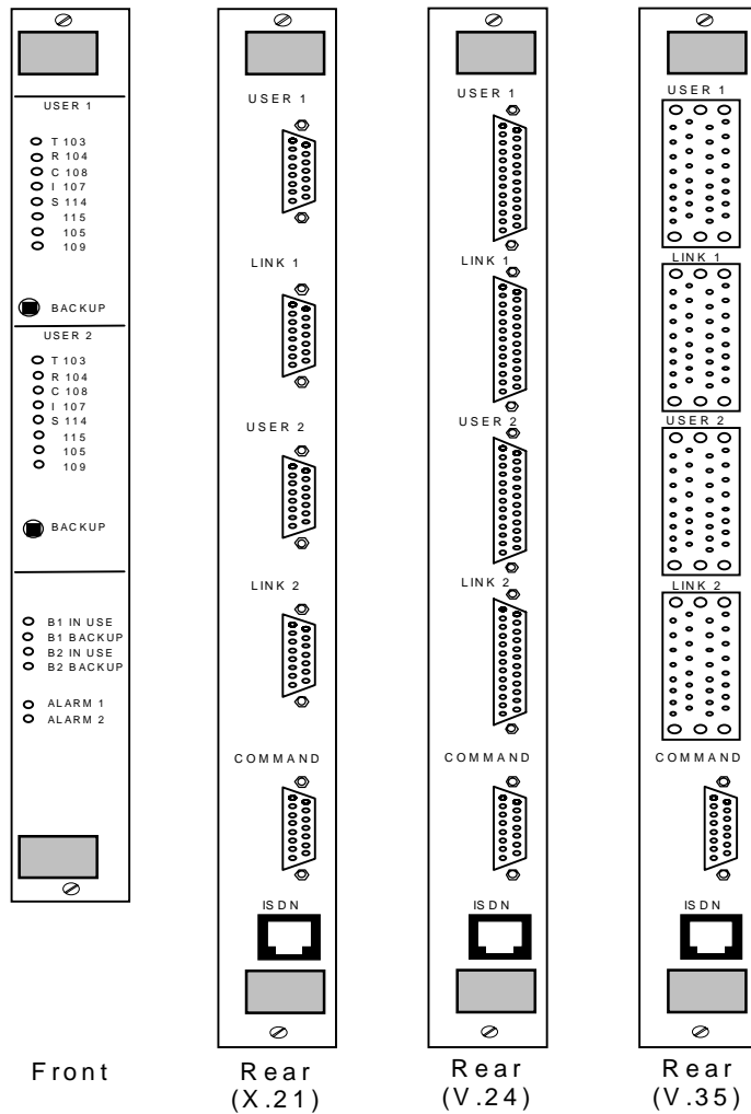
Figure 2.1 Front and rear Panel Layout
