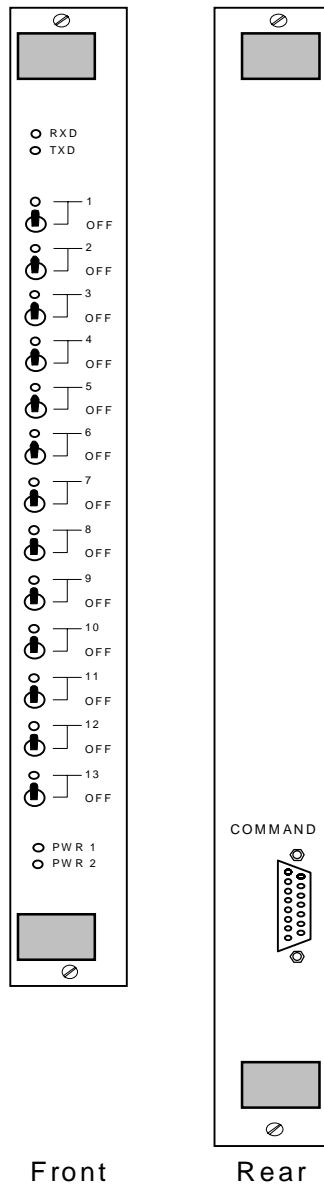
Figure 3.1 Front and Rear Panels of the Manager Card
