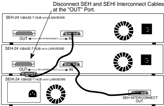
Figure 3-2. Disconnecting the HubSTACK Interconnect Cable
