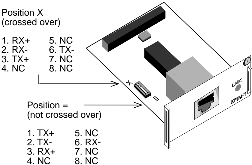
Figure 2-3. EPIM-T Pinouts
