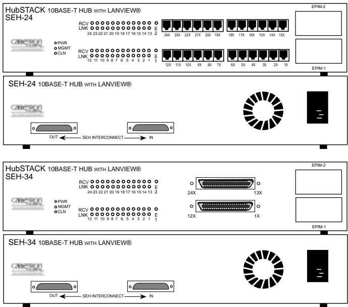
Figure 1-1. The SEH-24 and SEH-34
