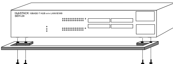
Figure 3-3. Attaching the Strain Relief
