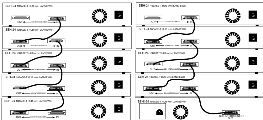
Figure 3-1. Stacking the SEH
