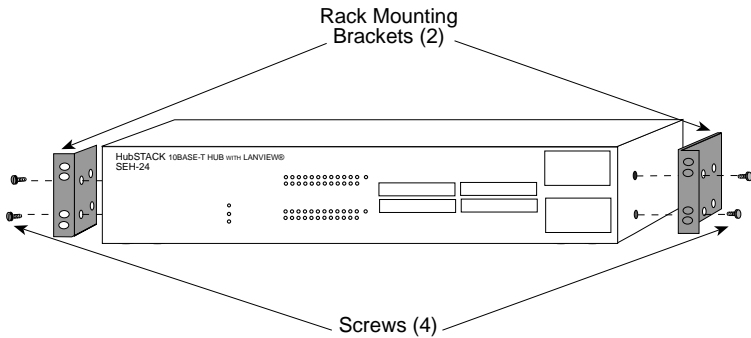
Figure 3-4. Installing the Rack Mount Brackets
