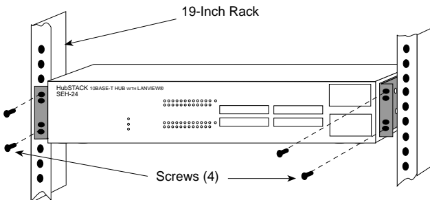
Figure 3-5. Installing the SEH in the Rack
