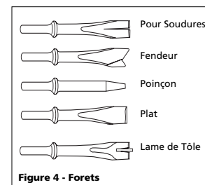
Figure 4 - Forets
