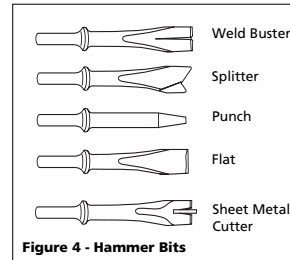
Figure 4 - Hammer Bits
